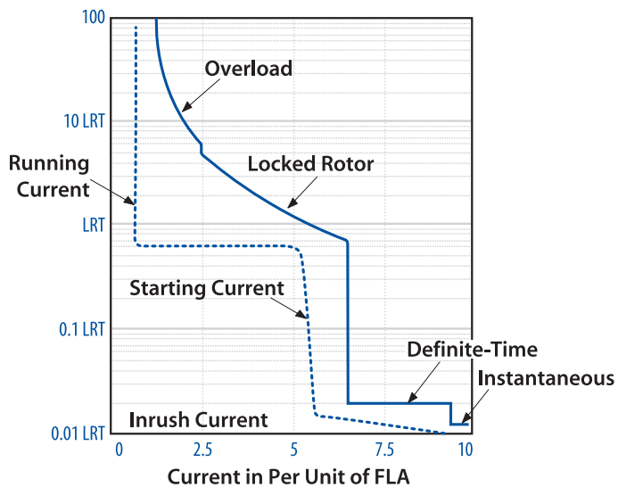
Motor characteristics plotted with motor starting current.
