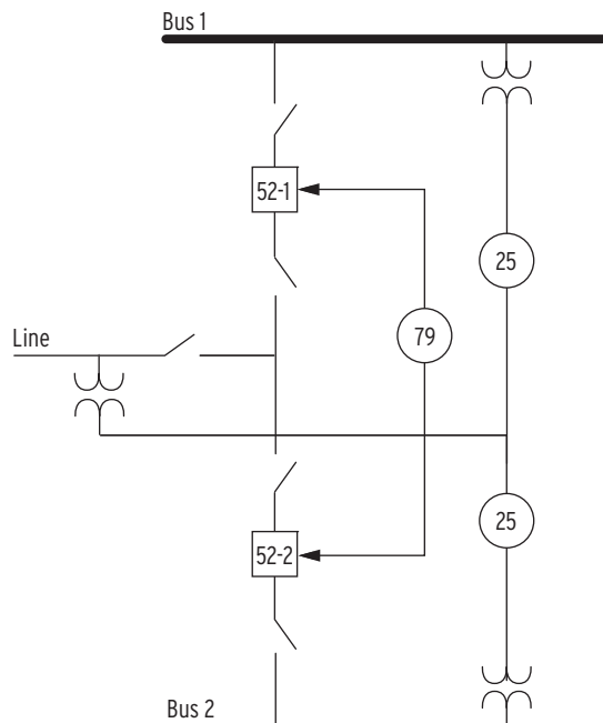
Figure 22 Two-Breaker Reclosing With Synchronism Check
