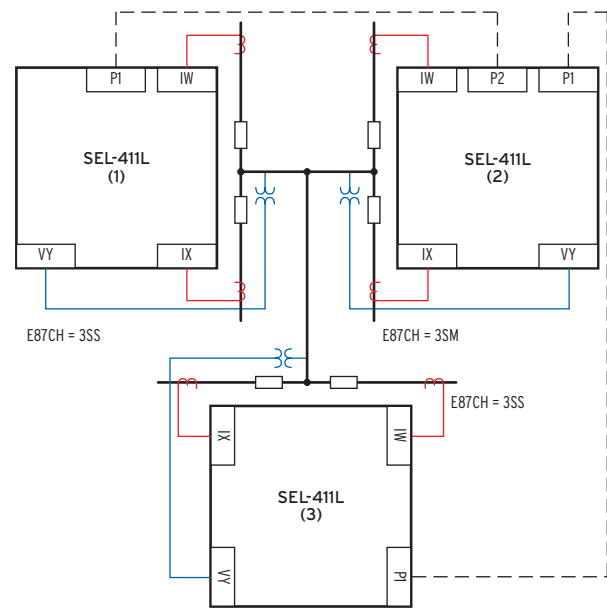
Figure 36 Three-Terminal Application Over Serial Channels With Relay 1 and Relay 3 as Slaves
