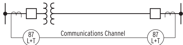
Figure 38 In-Line Transformer With Combined Line and Transformer Current Differential
