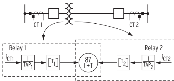
Figure 9 Compensation for In-Line Transformers at the Local Relay Allows the Algorithms to Remain Unchanged
