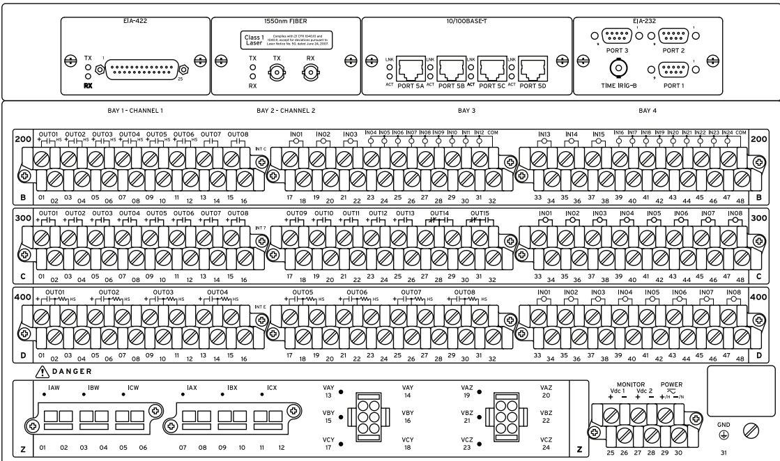
6U Rear Panel, Connectorized Terminal Block, Three (INTC, INT7 and INTE) I/O Board Option
