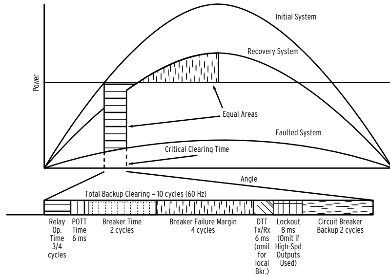
Figure 20 Combining High-Speed Tripping (87L, 21), MIRRORED BITS Communications, and High-Speed Open-Pole Detection in the SEL-411L Relay Provides for Faster Total Clearing Time
