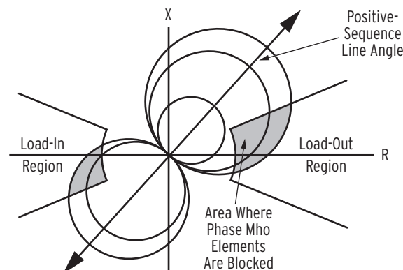
Figure 19 Load-Encroachment Logic
