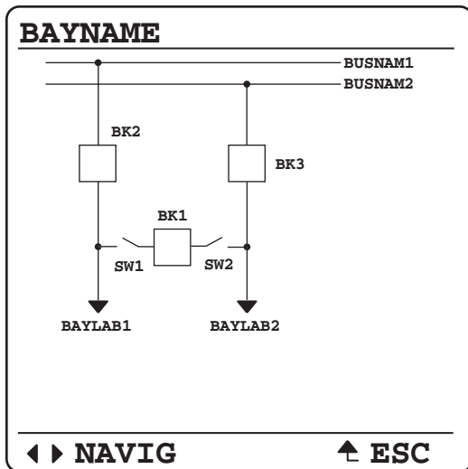
Figure 30 Breaker-and-a-Half
