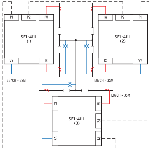
Figure 35 Three-Terminal 3SM Configuration With All Relays as Masters
