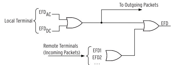
Figure 8 Combined External Fault Detector
