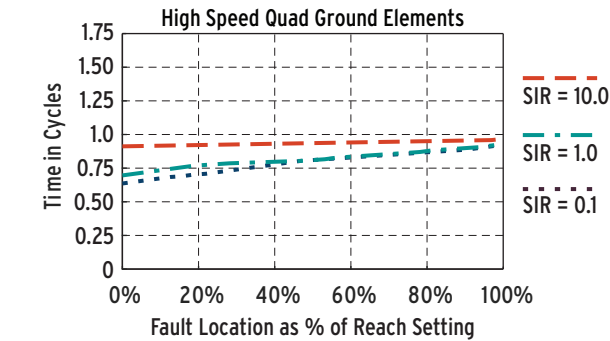
Figure 16 Quadrilateral Single-Phase-to-Ground Faults
