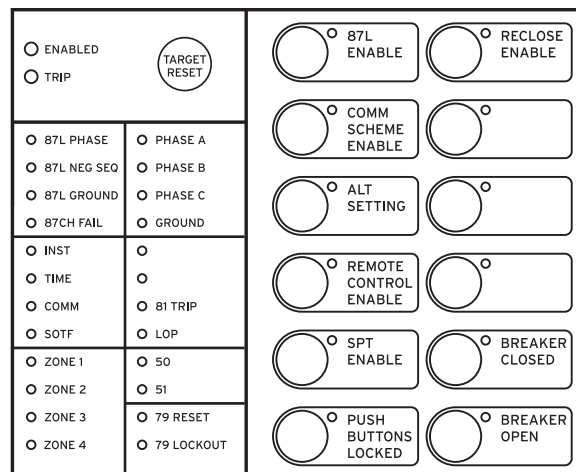
Figure 28 Factory Default Status and Trip Target LEDs (12 Pushbutton, 24 Target LED Option)
