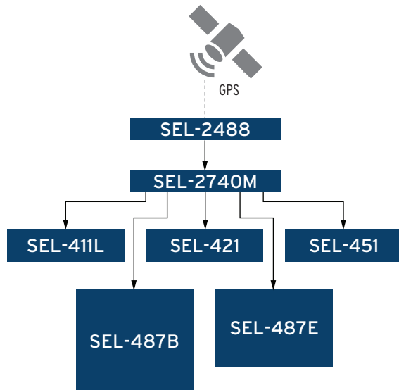
Figure 24 Example PTP Network
