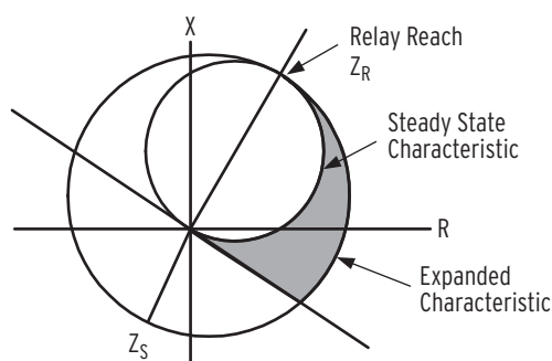
Figure 18 Mho Characteristic
