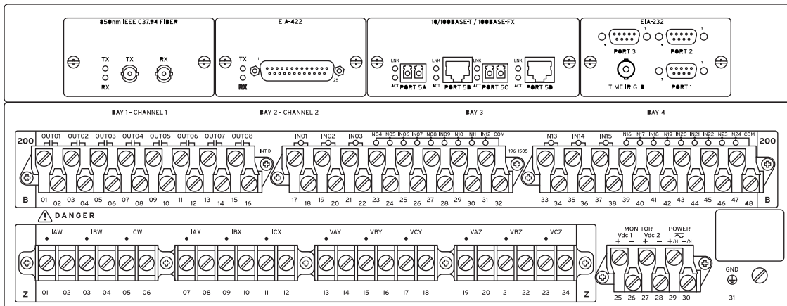
4U Rear Panel, Terminal Block, One INTD I/O Board Option
