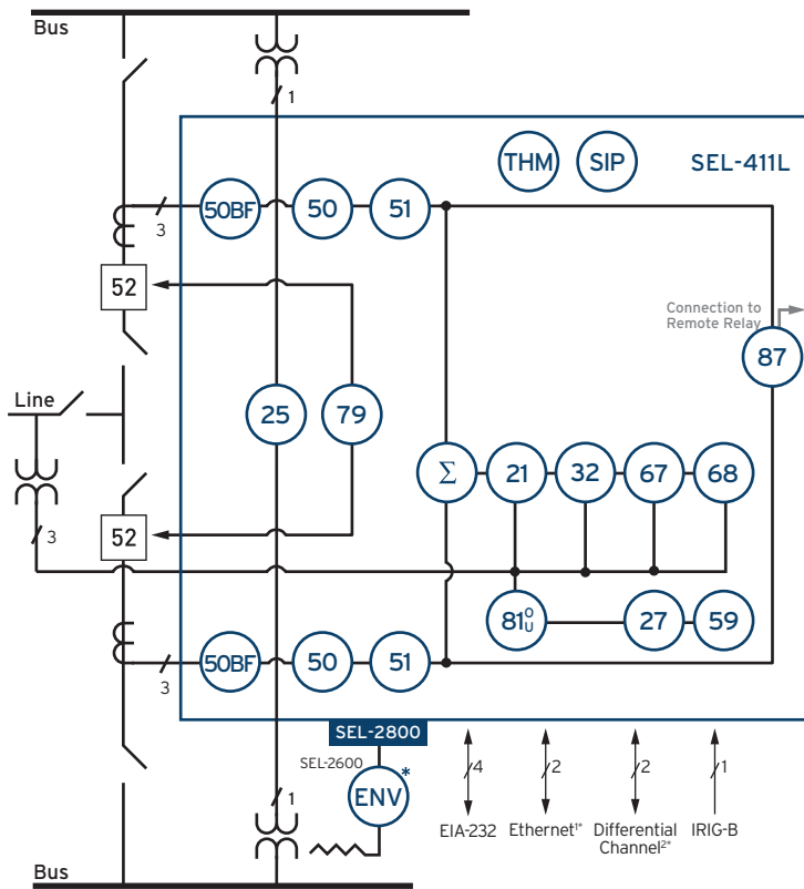
Figure 1 Functional Diagram
