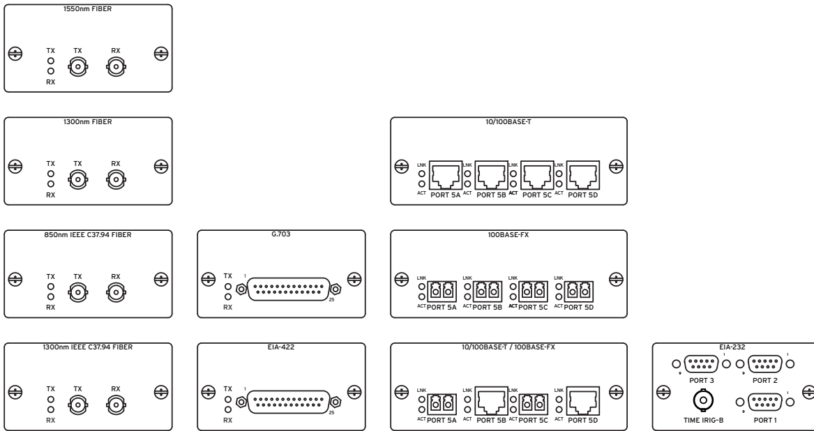
Figure 41 SEL-411L 87L Communications, Ethernet, and Serial Board Options
