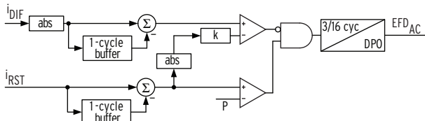
Figure 6 AC Saturation Path of the External Fault Detector
