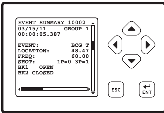
Figure 29 Factory-Default Front-Panel Display and Pushbuttons
