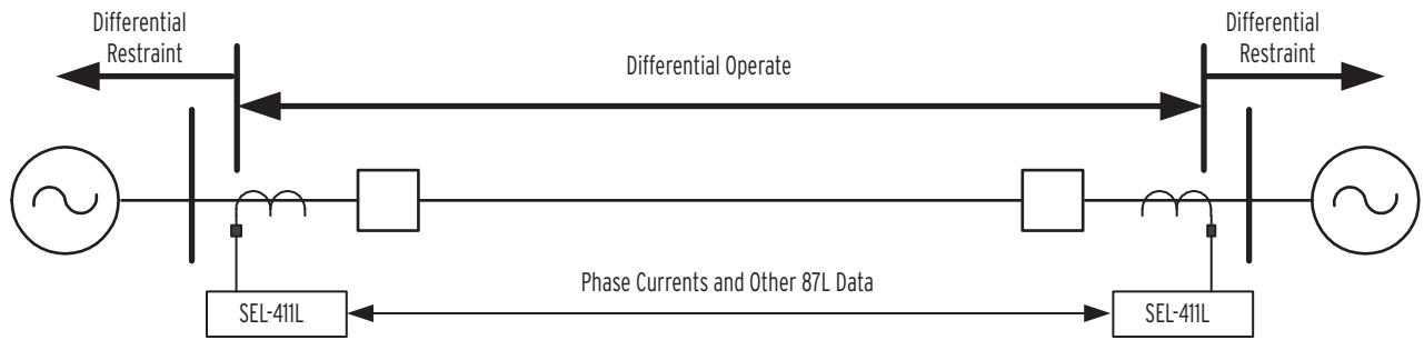
Figure 2 Differential Element Operate and Restraint Regions
