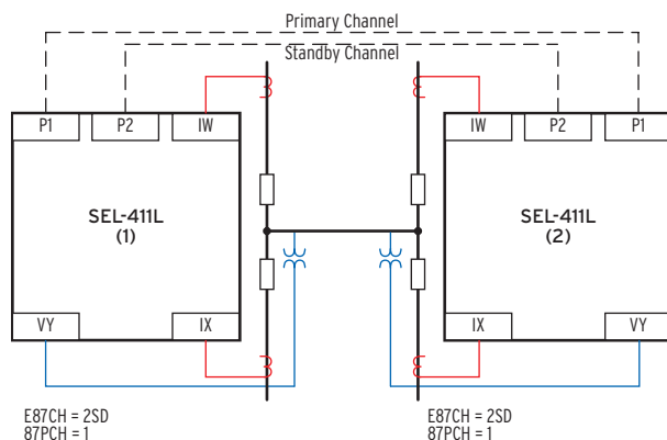
Figure 34 Two-Terminal 2SD Configuration With Both Line Ends Terminated on Dual-Breaker Buses and Port 1 Configured as Primary
