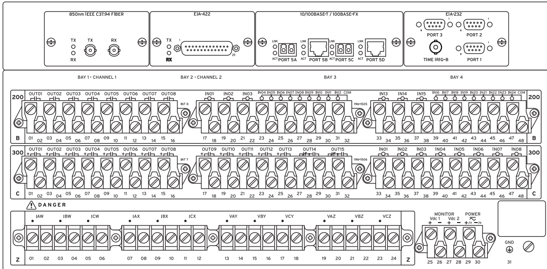
5U Rear Panel, Terminal Block, Two (INTD and INT7) I/O Board Option
