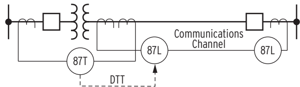
Figure 37 Preferred Application for Lines With Transformer
