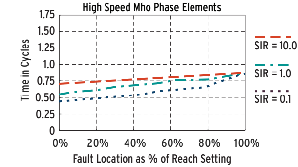
Figure 15 Mho Phase-to-Phase Faults
