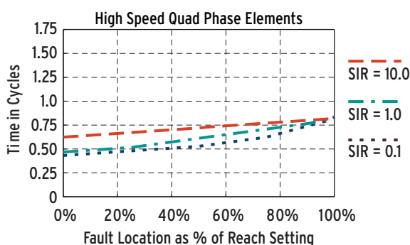
Figure 17 Quadrilateral Phase-to-Phase Faults
