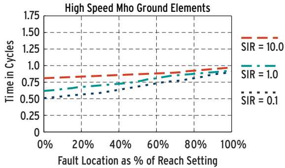
Figure 14 Mho Single-Phase-to-Ground Faults
