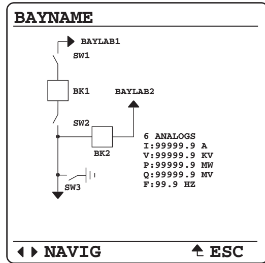
Figure 31 Ring Bus With Ground Switch
