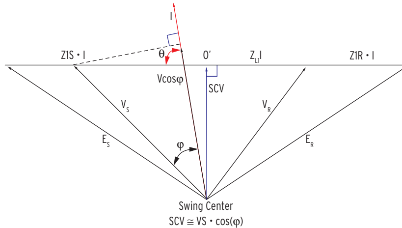
Figure 21 Applying V_S to Approximate the Swing Center Voltage Provides an Accurate Local Quantity to Detect Power Swings
