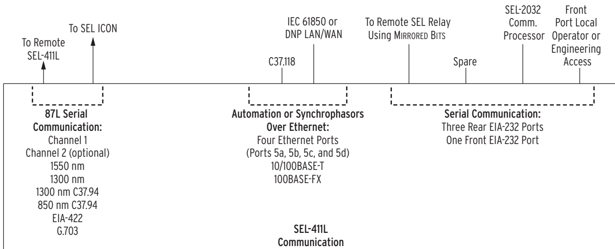
Figure 23 System Functional Overview
