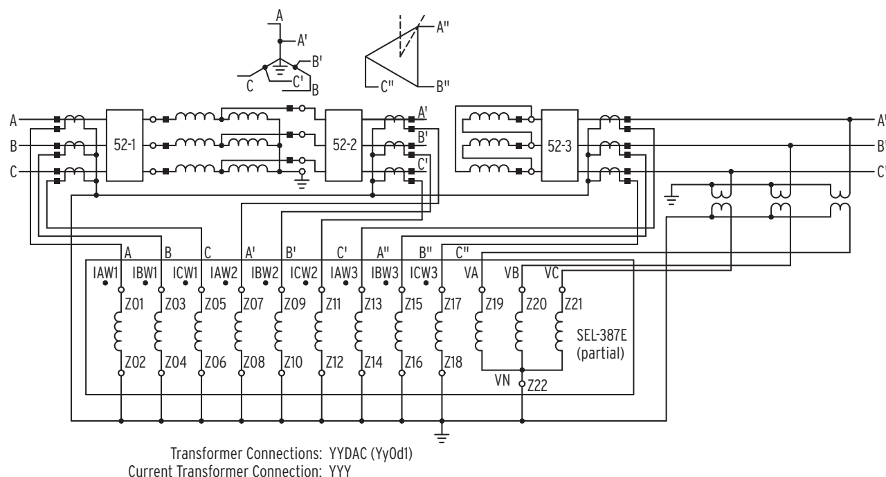
Figure 8 Typical AC Connection Diagram, Three-Winding Autotransformer Application
