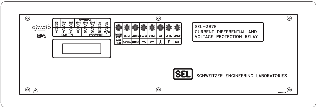
Figure 12 SEL-387E 3U Panel-Mount Front Panel
