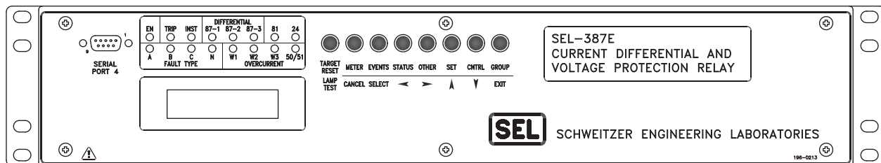
Figure 10 SEL-387E 2U Rack-Mount Front Panel
