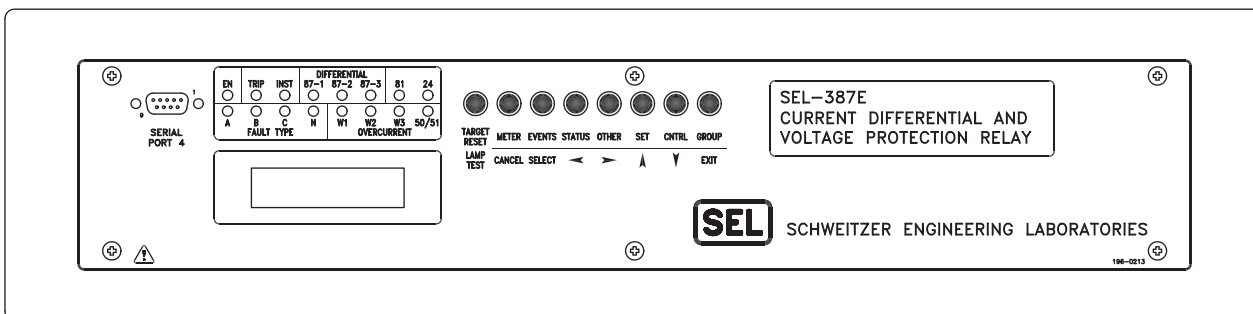
Figure 11 SEL-387E 2U Panel-Mount Front Panel
