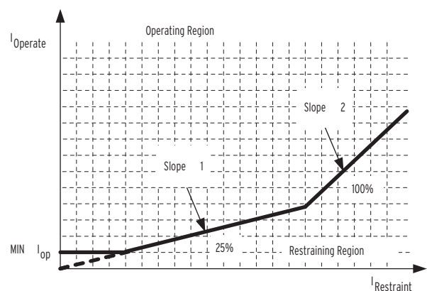
Figure 2 Dual-Slope Percentage Differential Restraint Characteristic
