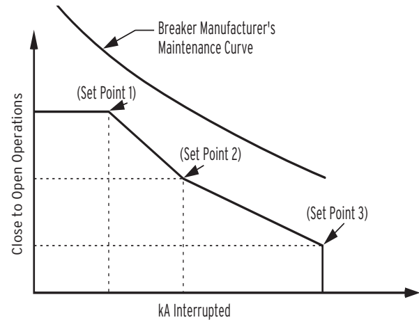
Figure 4 Breaker Contact Wear Curve and Settings
