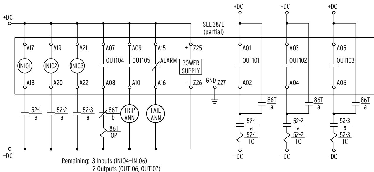
Figure 9 Typical DC Connection Diagram, Three-Winding Transformer Application
