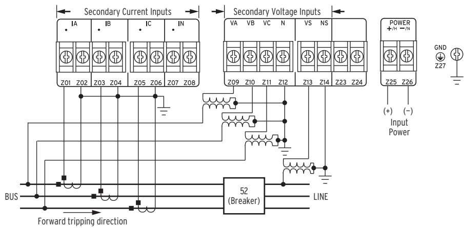
Figure 26 Example SEL-311C Wiring Diagram (Wye-Connected PTs; Synchronism-Check Voltage Input) (2 of 2)
