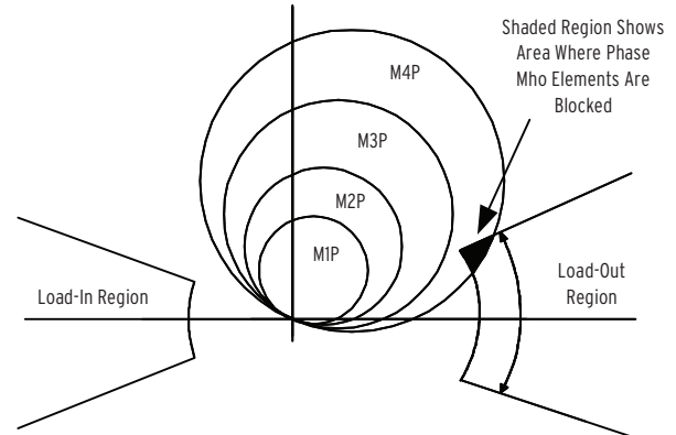
Figure 4 Load-Encroachment Characteristic
