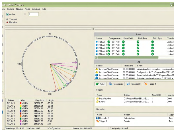
Figure 11 SEL-5078 SYNCHROWAVE Console Software Provides a Real-Time, Wide-Area Visualization Tool
