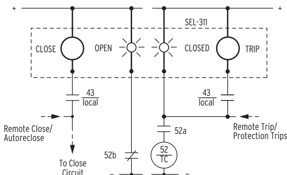
Figure 14 Optional SafeLock Trip/Close Pushbuttons and Indicating LEDs
