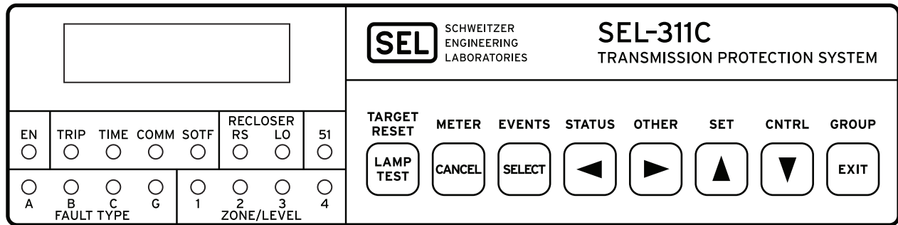
Figure 25 Status and Trip Target LEDs, Front-Panel Display, and Pushbuttons
