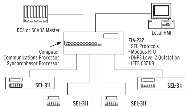
Figure 18 Typical Serial Communications Architecture
