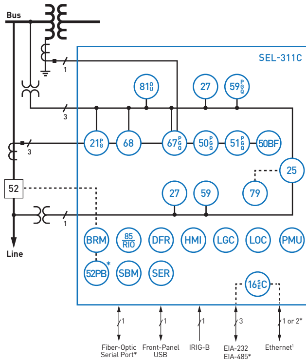
Figure 1 Functional Diagram
