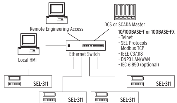
Figure 19 Typical Ethernet Communications Architecture
