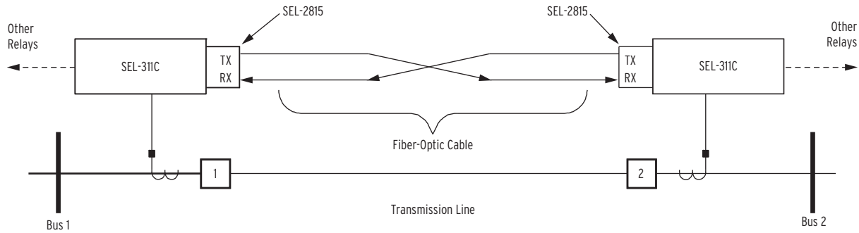
Figure 23 Integral Communications Provide Secure Protection, Monitoring, and Control
