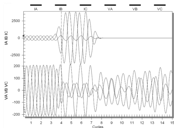
Figure 7 SEL-5601 Graph Event Reports
