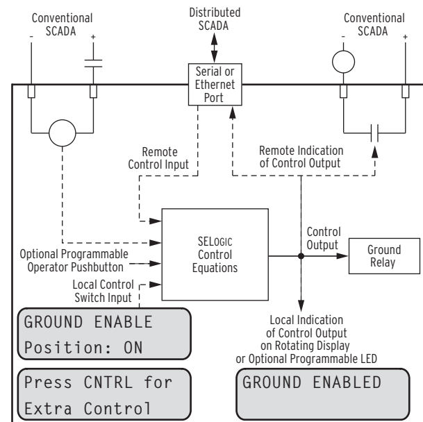
Figure 15 Local and Remote Control Using SELogic Control Equations (Ground Relay Example)
