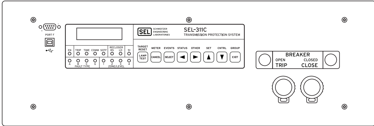
Figure 27 SEL-311C Horizontal Front-Panel Drawing (3U)
