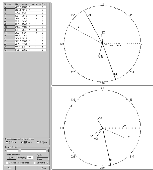
Figure 8 SEL-5601 Phasors
